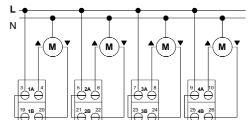
h Connection of the loads (device K.NAO.01O.20N.EU used as 16-fold binary output)
