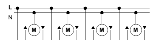
i Connection of the loads (device K.NAO.01O.20N.EU used as 8-fold blind actuator)
