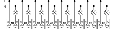
h Connection of the loads (device K.NAO.01O.20N.EU used as 16-fold binary output)
